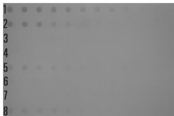
Fig. 5. Dot-blot of hemagglutinin in nanoparticles prepared by the emulsion and the double emulsion methods: lane 1, hemagglutinin; lane 2 dissolution control; lanes 3–5 emulsion method (E) (lane 3, first filtrate, lane 4, second filtrate, lane 5, washed and dissolved nanoparticles); lanes 6–8 double emulsion method (EE) (lane 6, first filtrate, lane 7, second filtrate, lane 8, washed and dissolved nanoparticles) (for details see Section 2).
