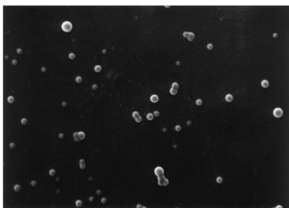
Fig. 1. Scanning electron micrograph of PLGA nanoparticles prepared by the emulsion method (1 \mu\text{m} =17 mm).
