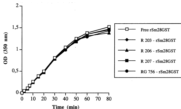
Fig. 3. Enzymatic activity of the entrapped rSm28GST released from microparticles. The glutathione S-transferase activity catalyzed by entrapped rSm28GST release from microparticles (closed symbols) was compared with that catalyzed by free rSm28GST (open symbol) in over time. The protein concentration (3.5 pmoles/well) was identical for each preparation.
