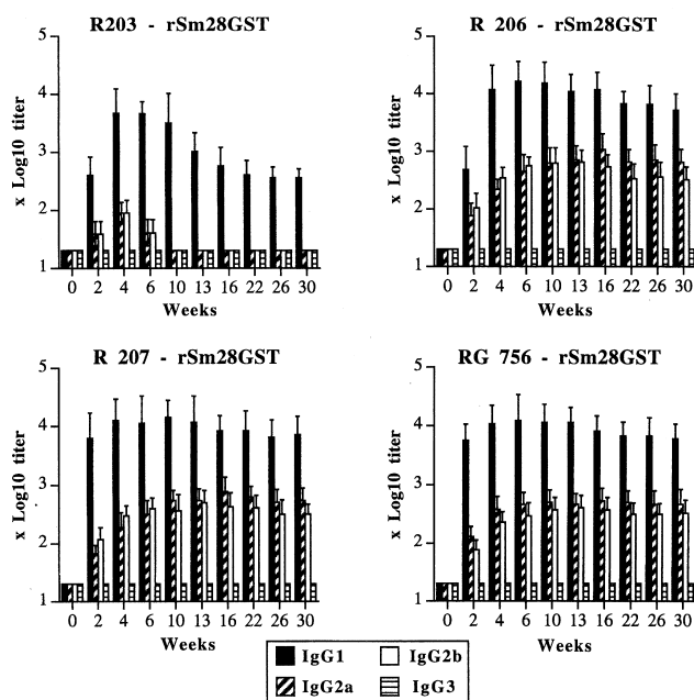
Fig. 4. Antibody isotype profiles elicited after immunization with rSm28GST entrapped in microparticles. Mice were immunized with R 203, R 206, R 207 or RG 756 microparticles. Anti-rSm28GST IgG1, IgG2a, IgG2b and IgG3 titers were determined at the indicated time points for individual serum from 10 BALB/c mice per group, before (week 0) and after immunization (from week 2). Results are expressed as titer mean values \pm standard deviation of the mean (S.D.). Titers are expressed as log 10 of the maximal dilution of the antiserum which gave an absorbance reading three-fold higher than background. The results shown are from one representative experiment of three.
