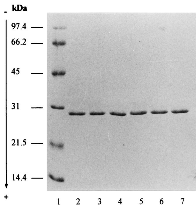
Fig. 2. Coomassie R 250-stained SDS-PAGE of rSm28GST (1.0 \mu\text{g} ) released from spray-dried microparticles of R 203 (lane 3), R 206 (lane 4), R 207 (lane 5) and RG 756 (lane 6). Lane 1: molecular weight markers. Lanes 2 and 7: free purified rSm28GST.
