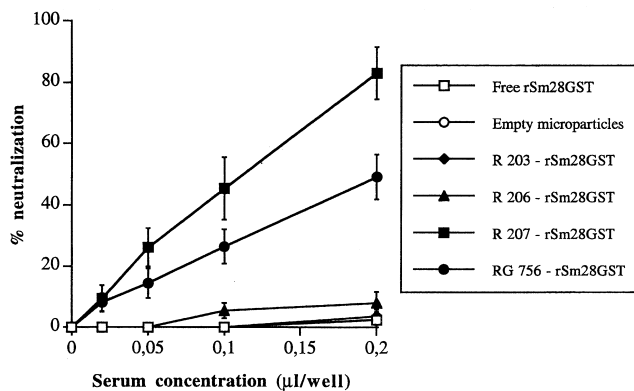
Fig. 5. Neutralization of the rSm28GST enzymatic activity by specific antiserum. The neutralizing activity was analyzed for pooled sera obtained 8 weeks after a single intraperitoneal administration of either rSm28GST-loaded R 203, R 206, R 207 or RG 756 microparticles, free rSm28GST or empty microparticles. Results are expressed as mean values ± S.D. of three separate experiments testing the neutralizing activity (%) of pooled sera for 10 mice in each group. The catalytic neutralization of rSm28GST (3.5 pmoles/well) was measured in the absence or presence of increasing concentrations of antisera. Sera expressing less than 10% neutralization at a concentration of 0.2 µl/well are considered as inefficient sera.
