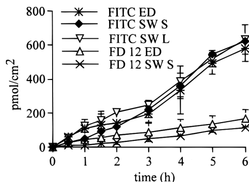
Fig. 3: Cumulative quantities of FITC and FD 12 after exponentially decaying (ED), square wave short (SW S) and square wave long (SW L) electroporation (ED = 10 \times 150\text{V} –150 msec separated by 30 sec; SW S = 891 \times 150\text{V} –1.68 msec and separated by 0.125 sec; SW L = 10 \times 150\text{V} –150 msec separated by 30 sec).
