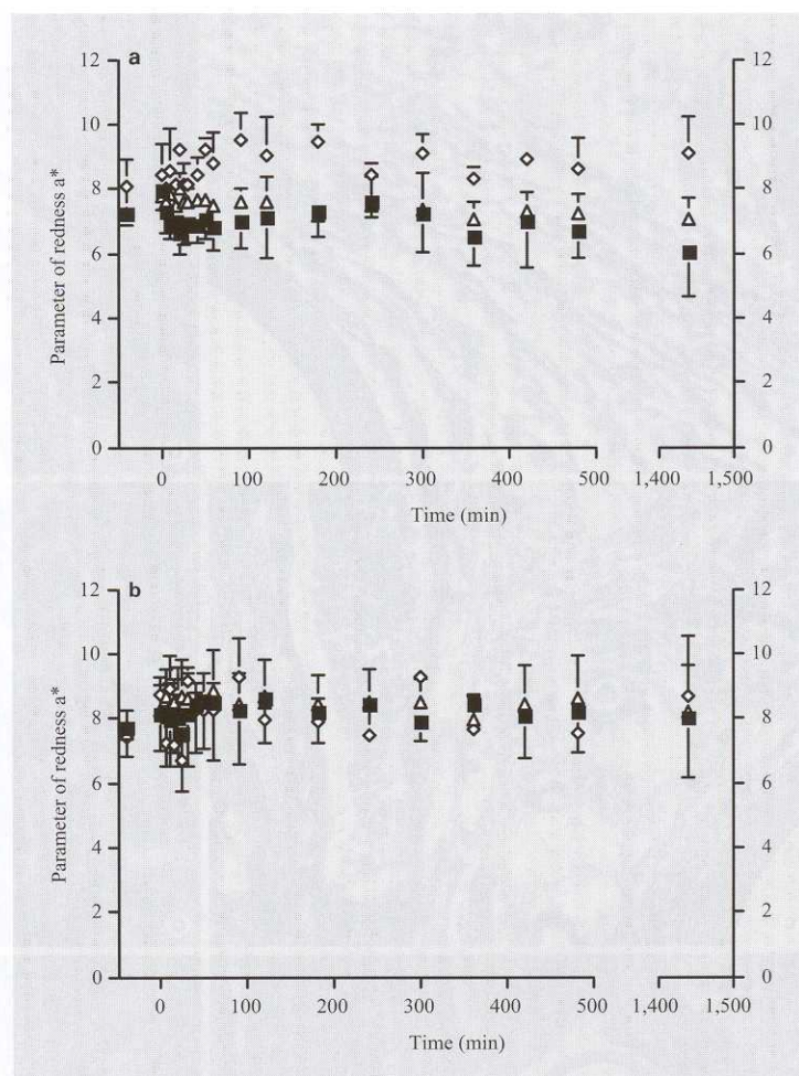
Fig. 3. Evaluation of erythema (redness a^* parameter) in rat as a function of time after insertion of microdialysis probe in subcutaneous tissue ( a ) and dermis ( b ). ■ = Control (no probe); △ = probe; ◇ = guide cannula. Mean \pm SEM, n = 8 .
