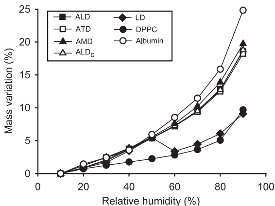
Fig. 5. Water adsorption isotherms of powders described in Table 1 as well as of spray-dried pure DPPC and albumin.
