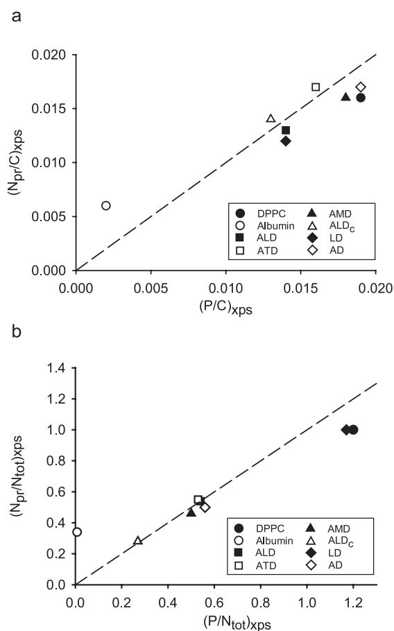
Fig. 2. Comparison of elemental concentration ratios determined by X-ray photoelectron spectroscopy: (a) (N_{pr}/C) vs. (P/C) and (b) (N_{pr}/N_{tot}) vs. (P/N_{tot}) . The mean of two or three measurements is presented for the powders described in Table 1, spray-dried pure DPPC and albumin as well as a powder made of albumin/DPPC 40/60 w/w (powder AD). Error bars are not shown for clarity. The dotted line represents the 1:1 relationship.
