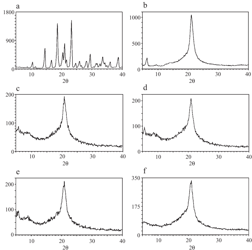
Fig. 4. X-ray diffraction diagrams of (a) spray-dried pure mannitol; (b) spray-dried pure DPPC; (c) powder ALD; (d) powder ALD c ; (e) powder AMD; (f) powder LD (see Table 1 for powder description). The diagram of powder ATD was similar to that of powder ALD or AMD and is not shown.
