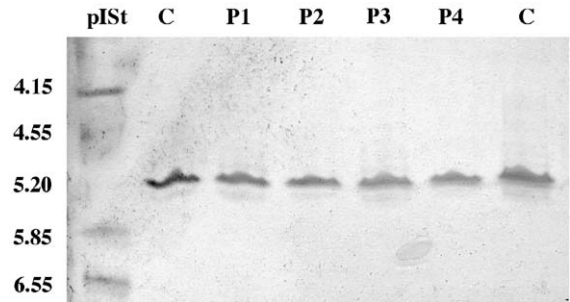
Fig. 2. hGH glycation assayed by isoelectric focussing. pISt= isoelectric point standards, C=hGH dissolved in buffer, P=hGH released from powders made of hGH/lactose/DPPC 10/30/60% w/w/w stored at 4 °C for 5 months (P1); 4 months (P2) or 2 months (P3) and from a powder containing trehalose (P4).
