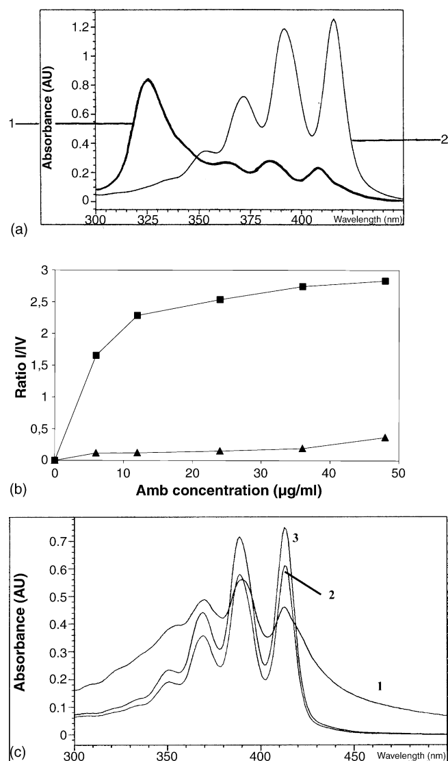
Fig. 2. (a) UV absorption spectra of amphotericin B at a concentration of 10 \mu\text{g/ml} in (1) aqueous solution (Fungizone ® ) and (2) DMSO. (b) Ratio of peak I to peak IV in the UV absorption spectra of amphotericin B as indicator of relative aggregation state as a function of amphotericin B concentration for Fungizone ® (■) and a 10% polymeric micelles solution PEG-p(CL-co-TMC) (▲) where amphotericin B, first dissolved in DMSO before its evaporation, was added to the polymer and then water (method B). (c) UV absorption spectra of 10 \mu\text{g/ml} amphotericin B encapsulated in 10% PEG-p(CL-co-TMC) by (1) method A (amphotericin B + polymer + water); (2) method B and (3) method C (amphotericin B, first dissolved in DMSO before its evaporation + polymeric micelles).
